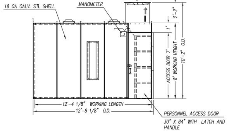
SIDE ELEVATION
