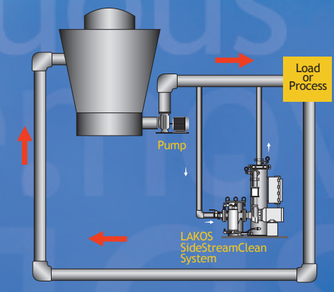
Side-Stream Protection
