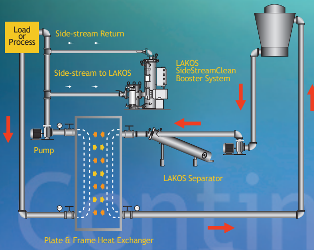
Full-Stream Protection
