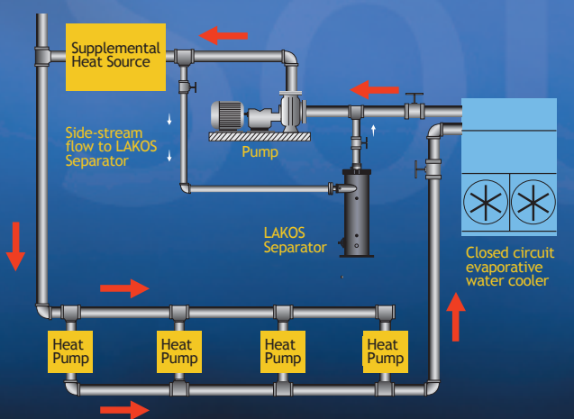
Side-Stream Protection
