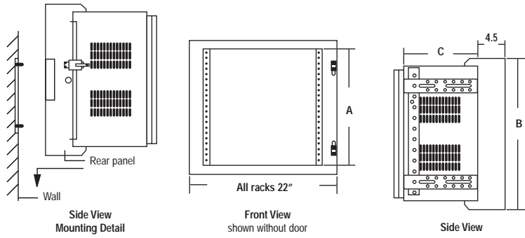
Plexi front door (SWRD-PLX) Perforated front door (SWRD-P) Solid front door (SWRD)
