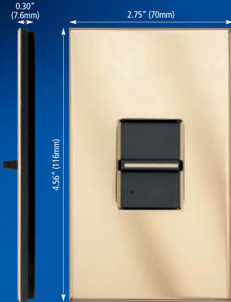
Shown actual size: NovaT ☆ slide-to-off dimmer with bright brass (BB) wallplate. Matte finish wallplate included with product.
