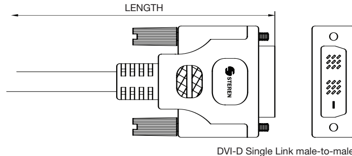
DVI-D Single Link male-to-male
