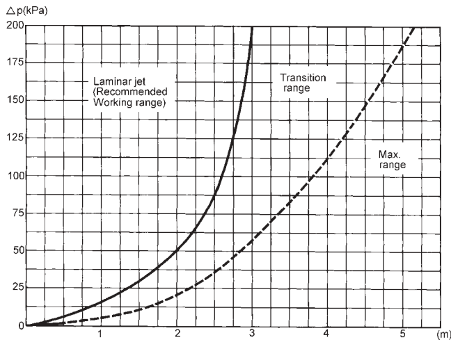
Cleaning range of 2 mm spray holes - LKRK
