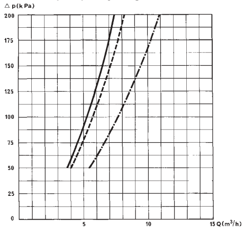
Pressure drop/capacity diagrams - LKRK
