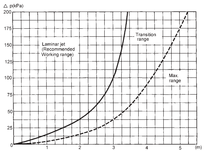
Cleaning range of 3 mm spray holes - LKRK
