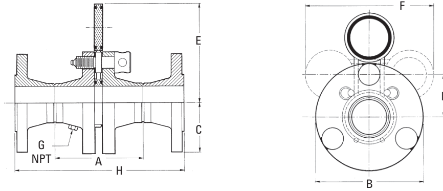
Model 15A/AF
