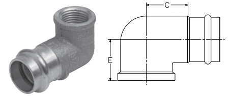
PC707-3 90° Elbow P x F – Cast
