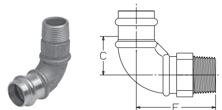
PC707-4 90° Elbow P x M – Cast
