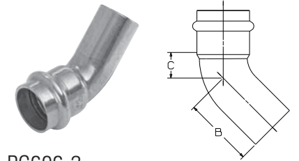
PC606-2 45° Elbow Ftg x P – Wrot
