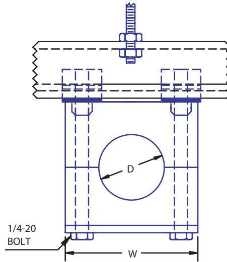
TYPICAL ASSEMBLY
