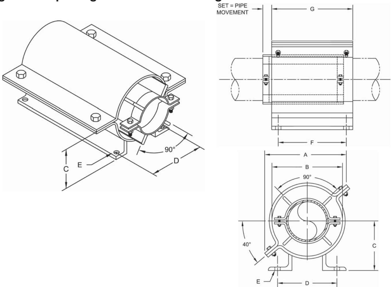
Fig. 420 - Pipe Alignment Guide — Long Traverse
