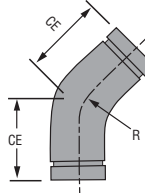
Figure 401 45° Elbow
