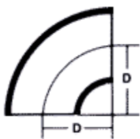
90° ELBOW/SHORT RADIUS
