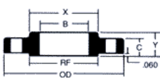
SLIP-ON
