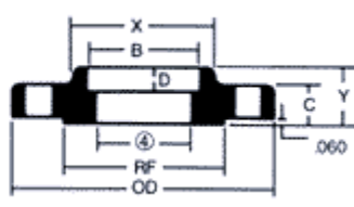
SOCKET WELD
