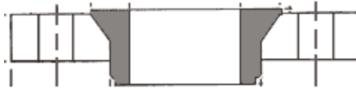
SLIP-ON STYLE
