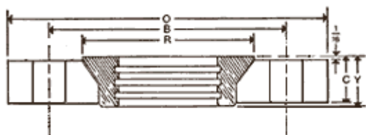
GROOVED STYLE
