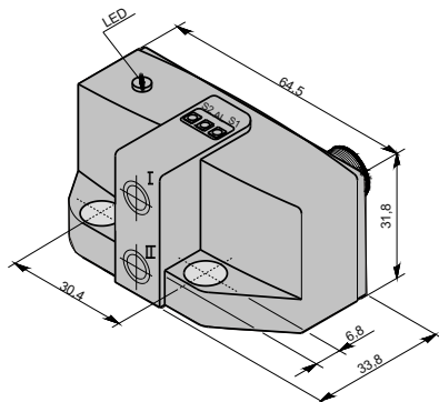
Sensor Block
