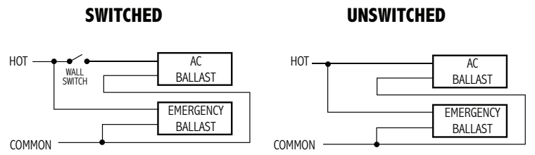
Primary circuit only. Lamp leads not shown.
