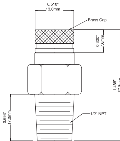
0.5" Test Plug
