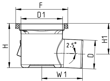
Side Outlet
