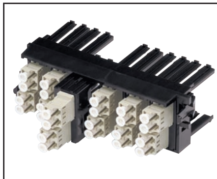
(Top): The 4U FiberExpress Ultra Patch Panel provides up to 288 fibers. (Left): Individual adapter modules feature a 1-inch pull out capability. (Right): Cassettes are easily installed or removed.
