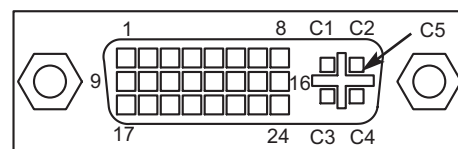
DVI-I FEMALE CONNECTOR
