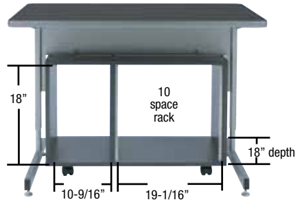
UCR under counter rack shown with SCD-42 (optional)
