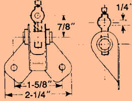
Typical Application Using Ball Joint and Damper Bracket
