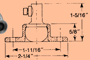
Ball Joint Damper Casting Cast Alloy
