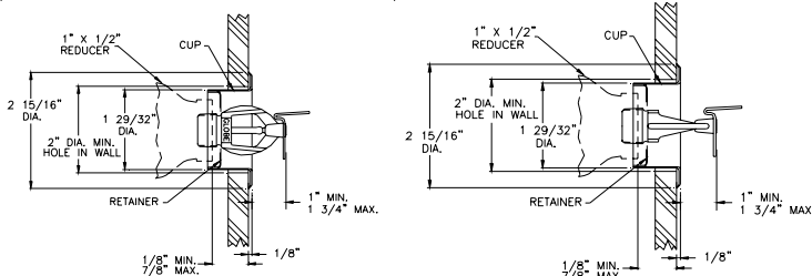
GL4230 & GL5630 GL5631 RECESSED HORIZONTAL SIDEWALLS
