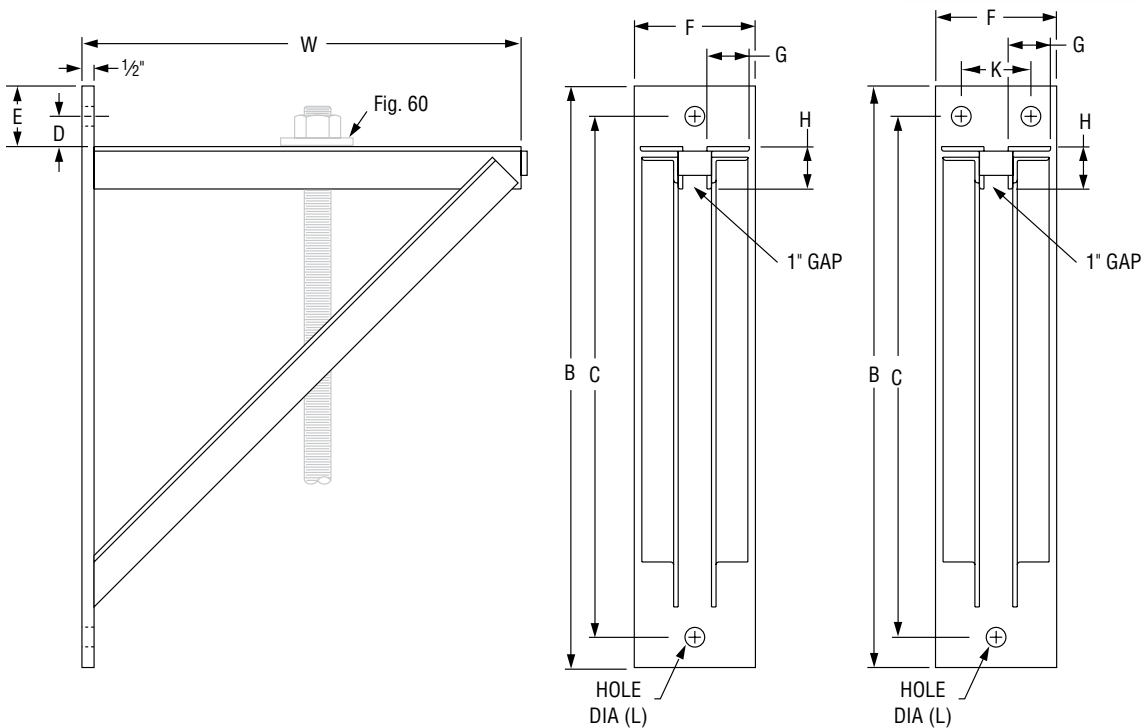
FIG. 199: LOAD (LBS) • WEIGHT (LBS) • DIMENSIONS (IN)
