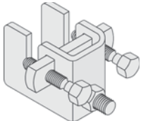
Fig. 825A Bar Joist Sway Brace Attachment Page 144
