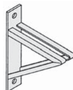
Fig. 30L, 30M, 30H Welded Bracket Light, Medium and Heavy Duty MSS-SP-69, Type 31 WW-H-171E, Type 32 Page 46
