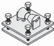
Fig. 328 Adjustable Pipe Roller Stand MSS-SP-69, Type 48 WW-H-171E, Type 47 Page 130
