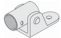
Fig. 910 Swivel Sway Brace Fitting Page 148
