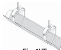
Fig. 1VT "V" Support Trough Page 20
