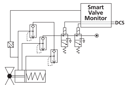
Fig. 2. HIPPS Configuration
