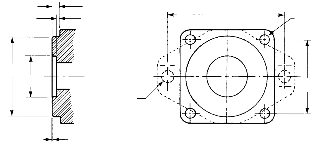
FIGURE 2 – DIMENSIONS OF STRAIGHT SHAFTS – WITHOUT THREAD
