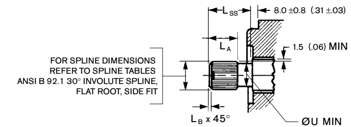
FIGURE 3 – DIMENSIONS OF 30° INVOLUTE SPLINE SHAFTS
