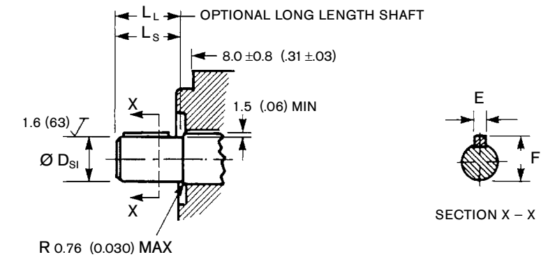
FIGURE 3 – DIMENSIONS OF 30° INVOLUTE SPLINE SHAFTS
