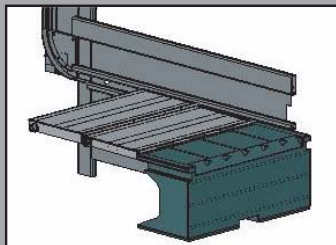
B) The follower cover extends and retracts with the blade.
