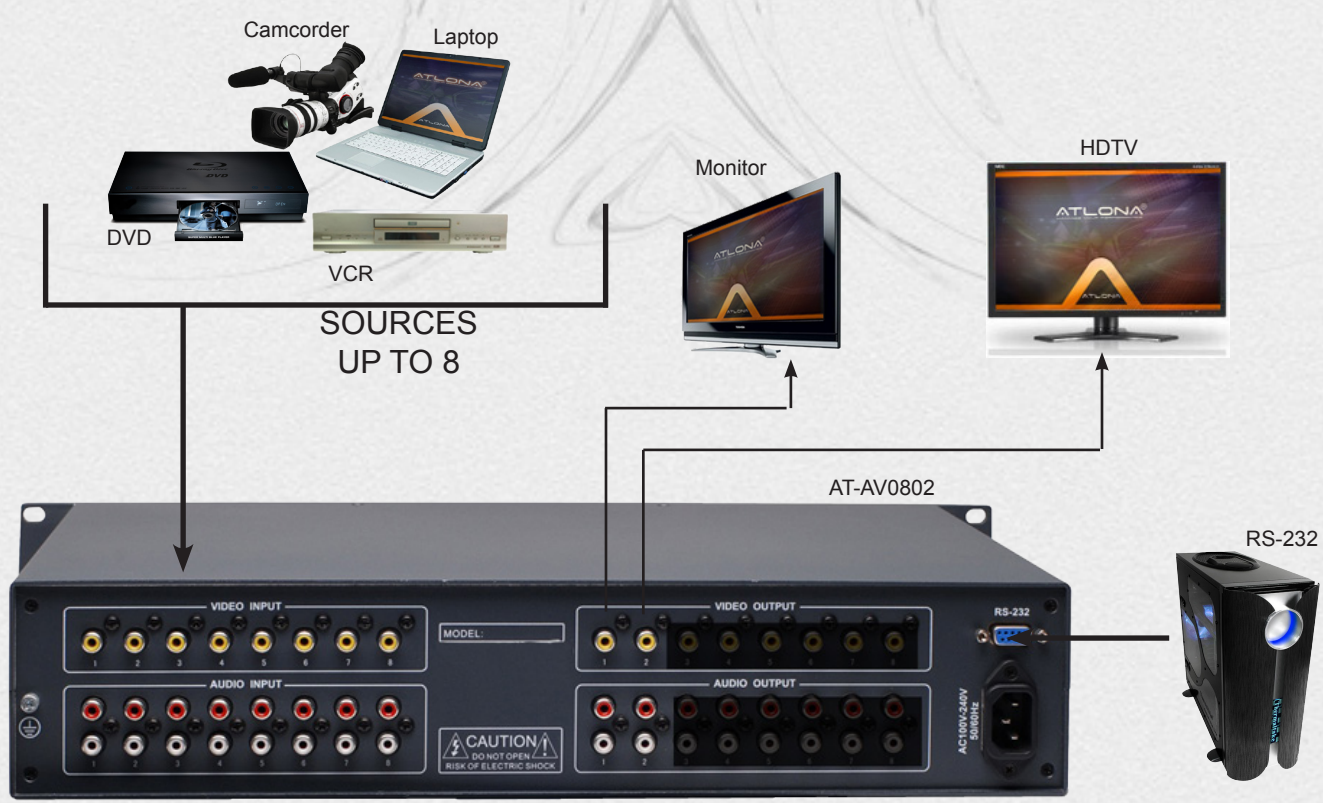
Connection Diagram
