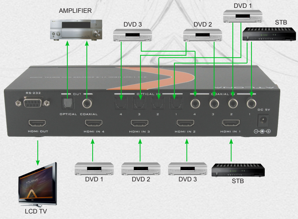
Connection Diagram:
