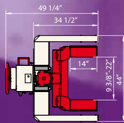
Adjustable forks
