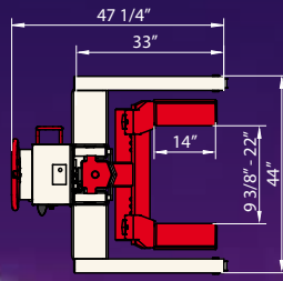
Adjustable forks
