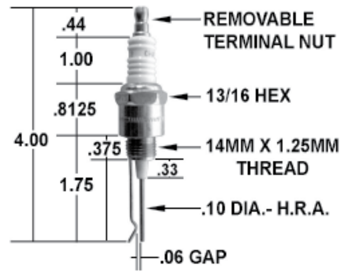
CA470 Replaces Auburn #: I-3 95% Alumina Ceramic
