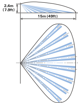
Coverage Pattern
