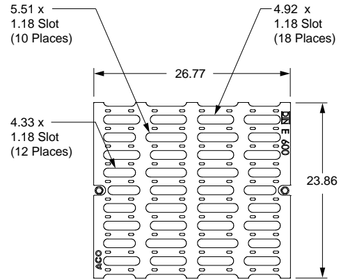
H20 Ductile Iron Grate Detail**
