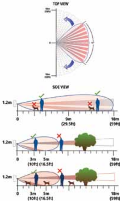
Coverage Pattern
