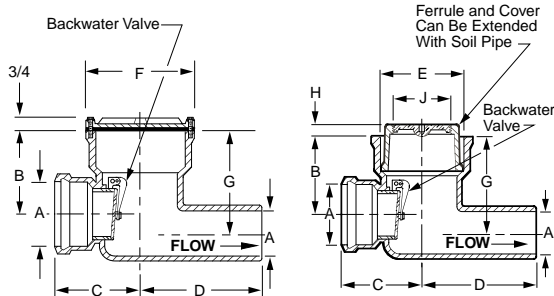
Fig. 7012 Bolted Cover
