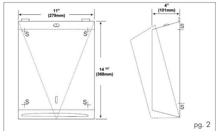
TOWEL DISPENSER SURFACE MOUNTED
