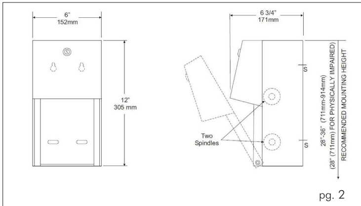
TOILET TISSUE DISPENSER
