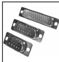
30-550 9-way 30-551 15-way 30-552 25-way "D" solder type connector plugs
