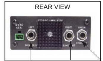
REAR VIEW Left 1/4" Speaker Output Jacks Right 1/4" Stereo Line Input
