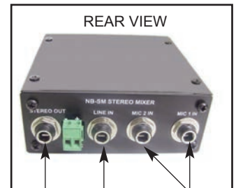
REAR VIEW 1/4" & 3.5mm Stereo Line Inputs 1/4" Stereo Line Output 1/4" Mic Inputs
