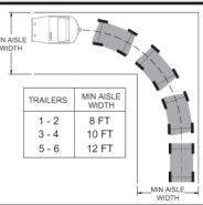
Minimum Aisle Width 8 feet (up to 3 Trailers)
