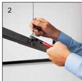
Step 2 – Suspend main beams with wire hangers
