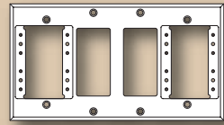
IPS-WP2Q 4 Gang Plate w/ 2 IPS and 2 Decora
