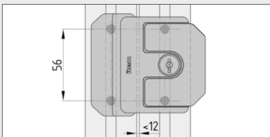
Profile bore grids for attaching Door Lock 6-8 Zn
