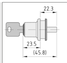
Mounting dimensions, locked and unlocked.
