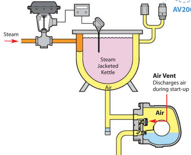
Air Vent Open Discharges air during start-up
