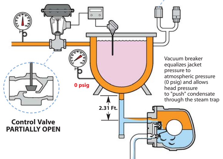
Vacuum Breaker OPEN
