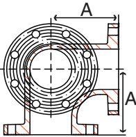
Fig. 38OE1 – 90° Side Outlet Elbow
