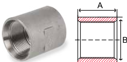
Fig. 29DC14 - 304 SS Recessed Drop Pipe Coupling
