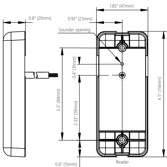
RBH-FR-360N Reader Mounting
