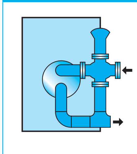
Figure 2 Modulating three-way diverting valve.
