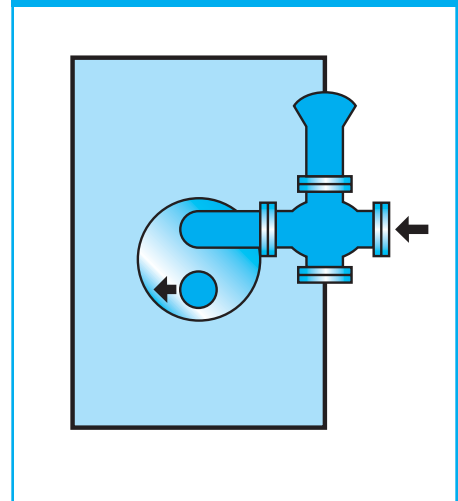
Figure 3 On-off modulating valve.
