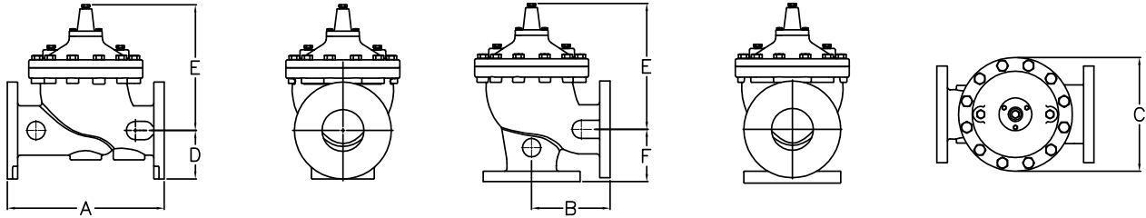
ANSI Valve Data (US Units)
