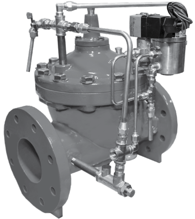
MS106-EDV-A-10507A Globe
