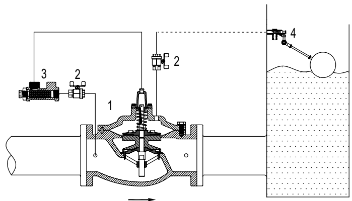
Schematic A-0608D
