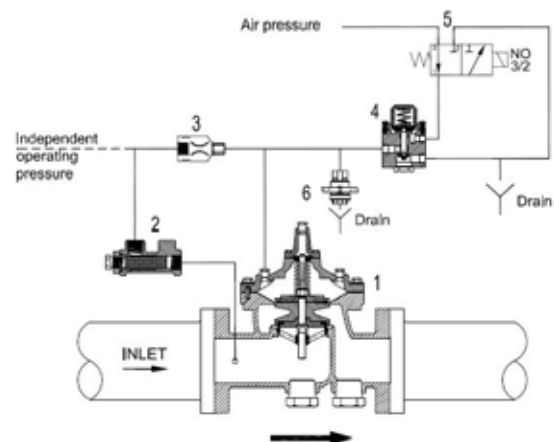
Schematic A-10506A
