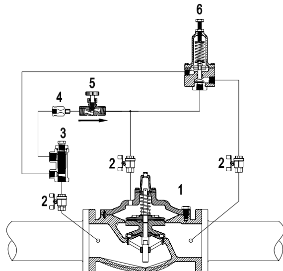
Schematic A-8700A
