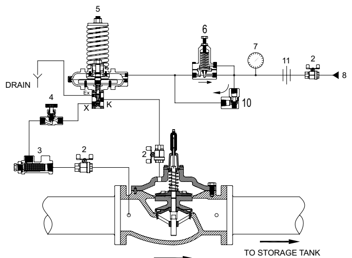
Schematic A-0415C
