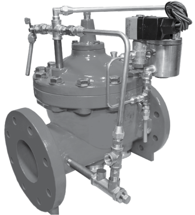
MS106-EPDV-A-10508A Globe
