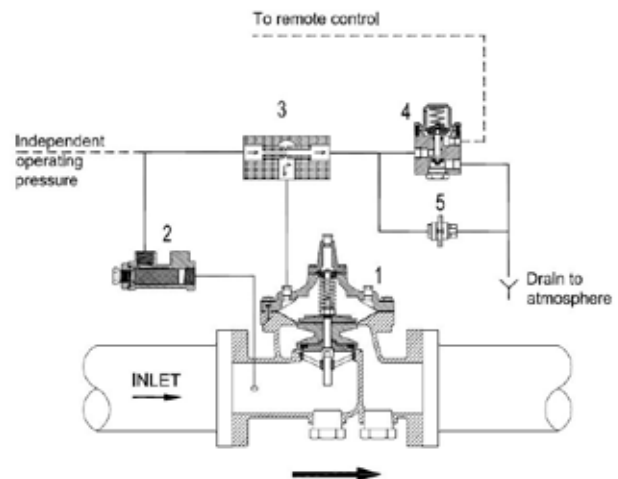
Schematic A-10508A
